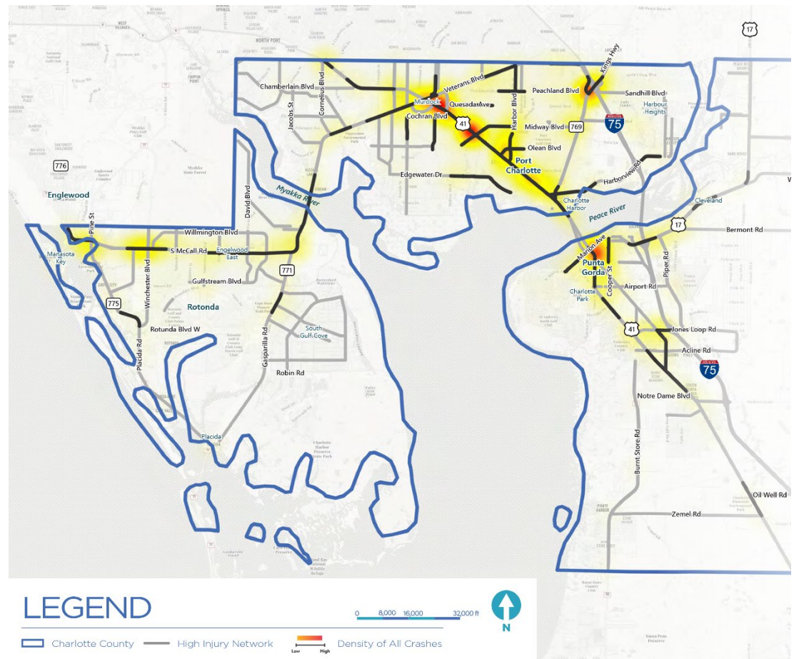
Figure 5-9. Charlotte County-Punta Gorda MPO Planning Area High Injury Network (HIN)
